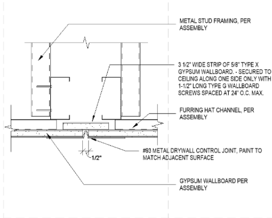
06 CEILING CONTROL JOINT - NOT RATED SCALE: 3" = 1'-0"
